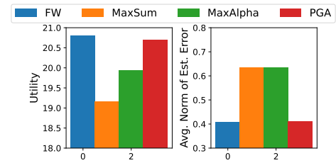
Fig. 8. Aggregate utility and average norm of estimation error in a simple example. Our proposed \mathcal{F}\mathcal{W} outperform all the competitors.
